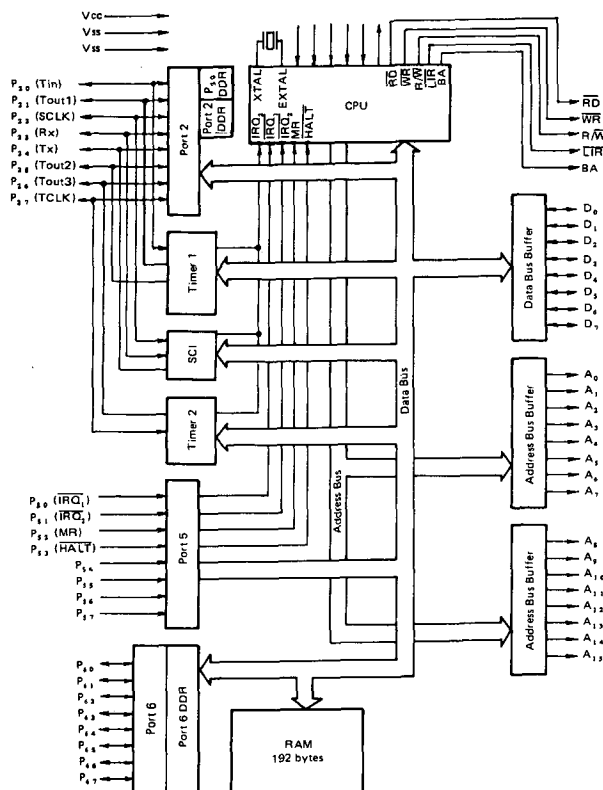
BLOCK DIAGRAM
