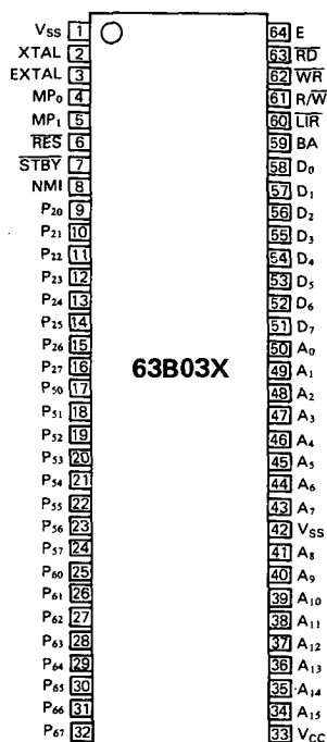
PIN CONFIGURATION
